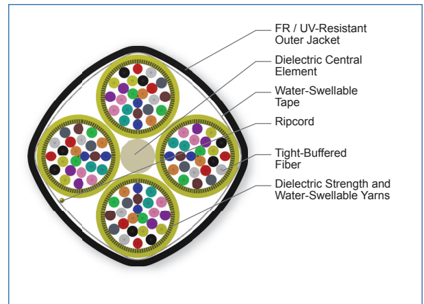
Cross Section of Part Number: 096Z8F-Y3131-29
