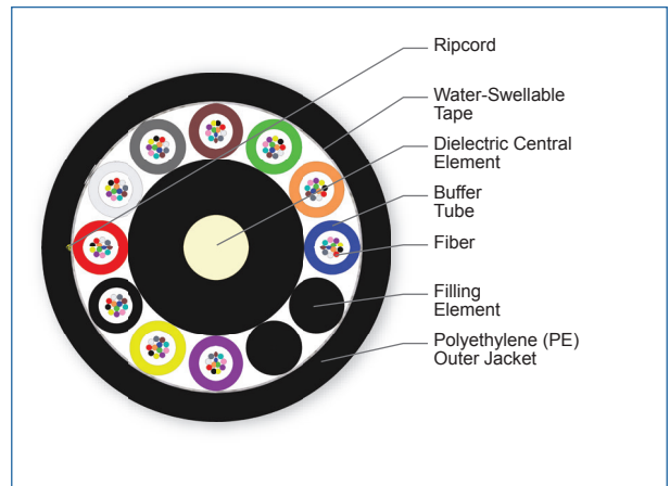
Cross Section of Part Number: 120TU4-T4180D20
