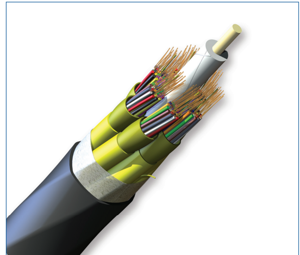
Part Number: 144E8F-Y3131-29
