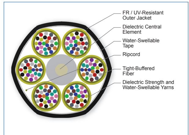
Cross Section of Part Number: 144E8F-Y3131-29
