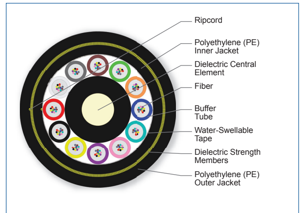
Cross Section of Part Number: 144EAE-T4401A20
