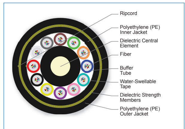
Cross Section of Part Number: 144EAE-T4A01A20
