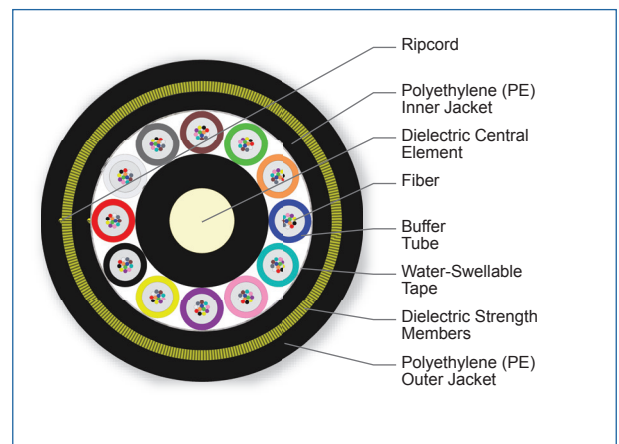
Cross Section of Part Number: 144EAE-T4C01A20
