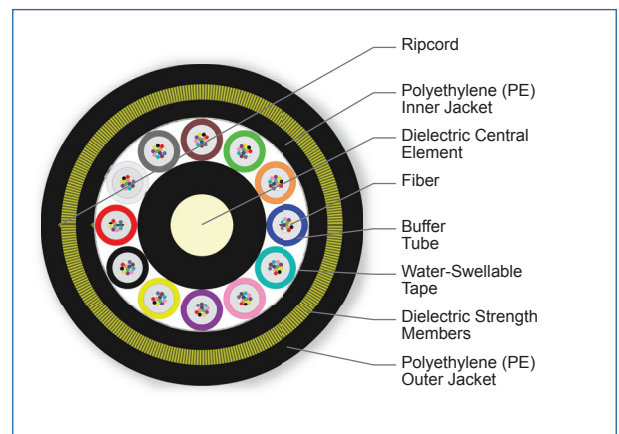
Cross Section of Part Number: 144EAE-T4F01A20
