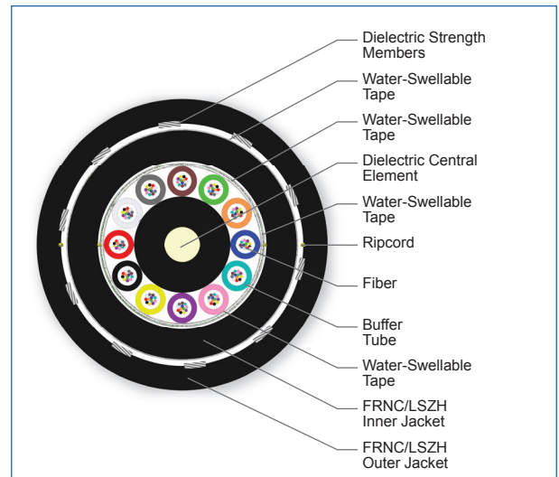
Cross Section of Part Number: 144EUL-T4601D2N
