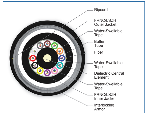
Cross Section of Part Number: 144EUZ-T4101DAN
