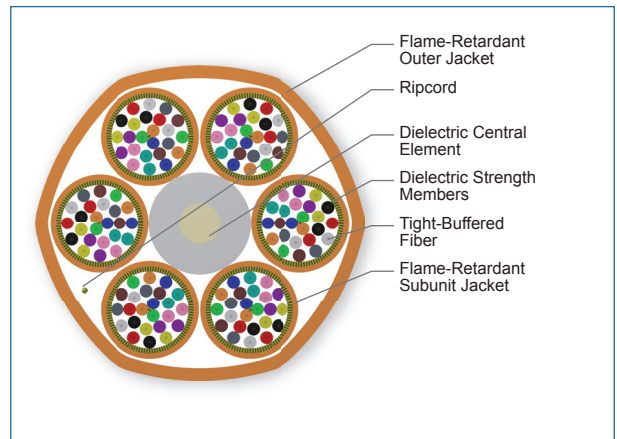
Cross Section of Part Number: 144K81-Y3130-24
