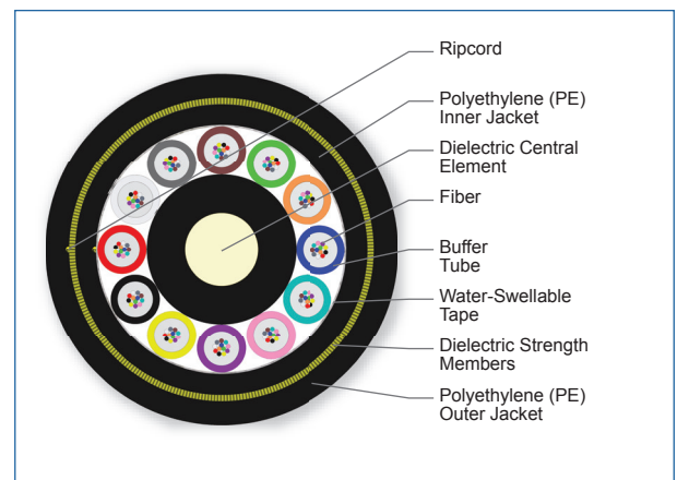
Cross Section of Part Number: 144KAE-T4430A20
