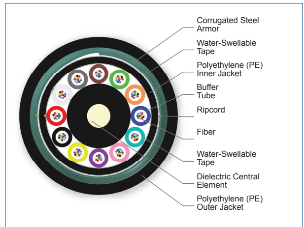
Cross Section of Part Number: 144KU5-T4130F20
