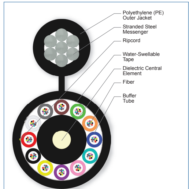
Cross Section of Part Number: 144KUA-T4130D20
