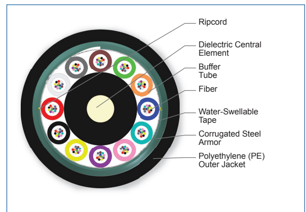
Cross Section of Part Number: 144KUC-T4130D20
