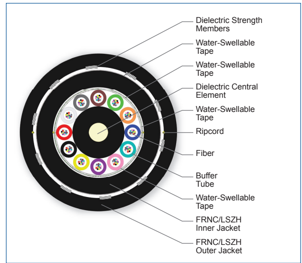
Cross Section of Part Number: 144KUL-T4630D2N
