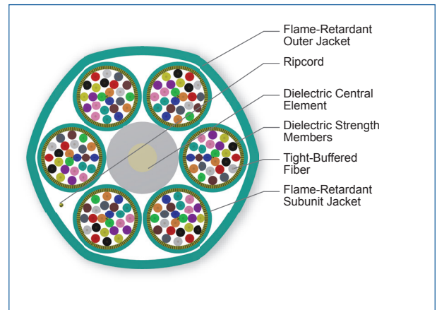
Cross Section of Part Number: 144T88-Y3191-29
