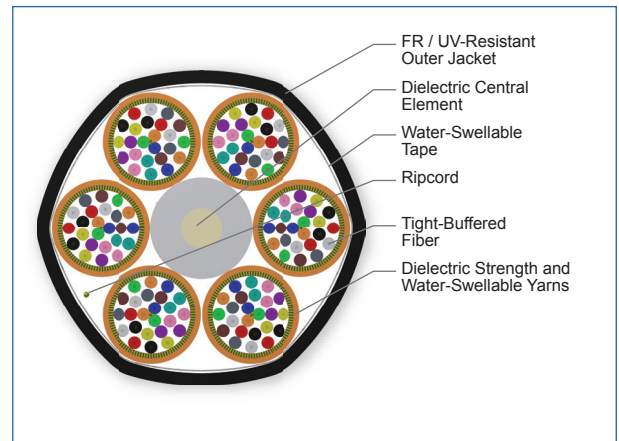
Cross Section of Part Number: 144T8F-Y3131-29
