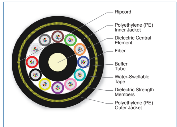
Cross Section of Part Number: 144TAE-T4A31A20
