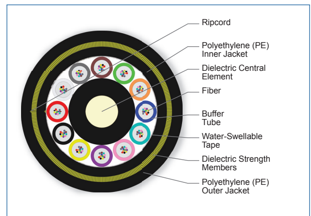
Cross Section of Part Number: 144TAE-T4C31A20
