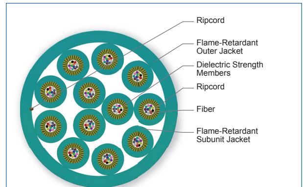
Cross Section of Part Number: 144TD8-T1390-20
