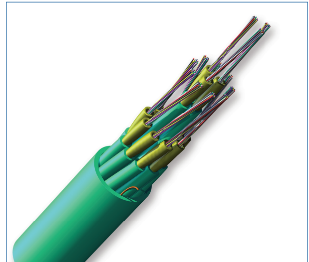
Part Number: 144TD8-T1390-20
