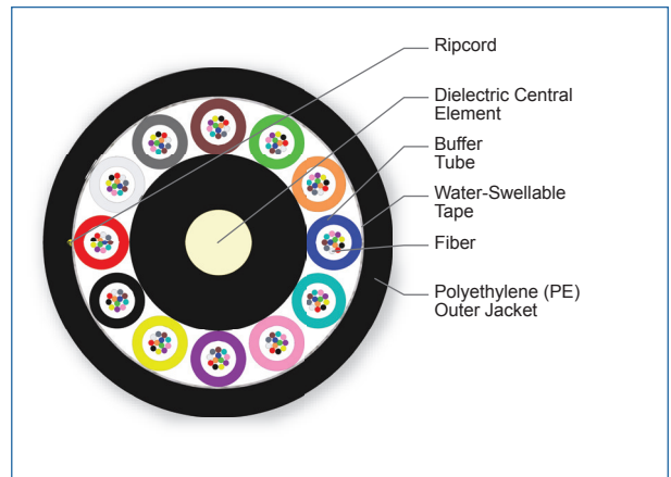
Cross Section of Part Number: 144TU4-T4180D20
