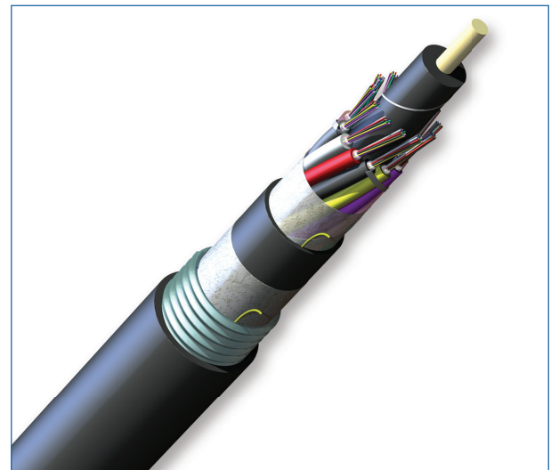
Part Number: 144TU5-T4131A20
