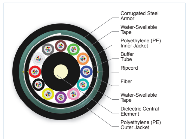
Cross Section of Part Number: 144TU5-T4131A20
