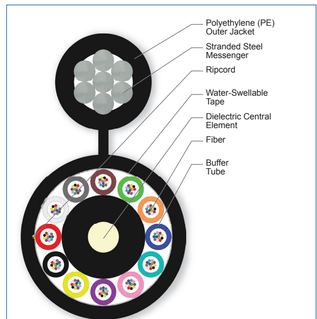
Cross Section of Part Number: 144TUA-T4131D20
