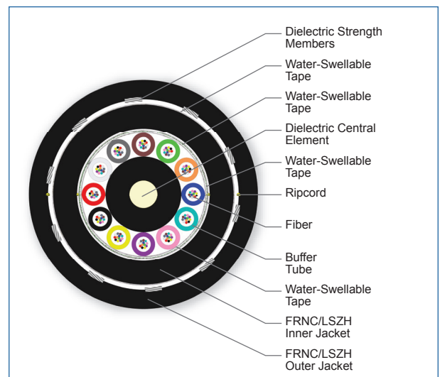
Cross Section of Part Number: 144TUL-T4691D2N
