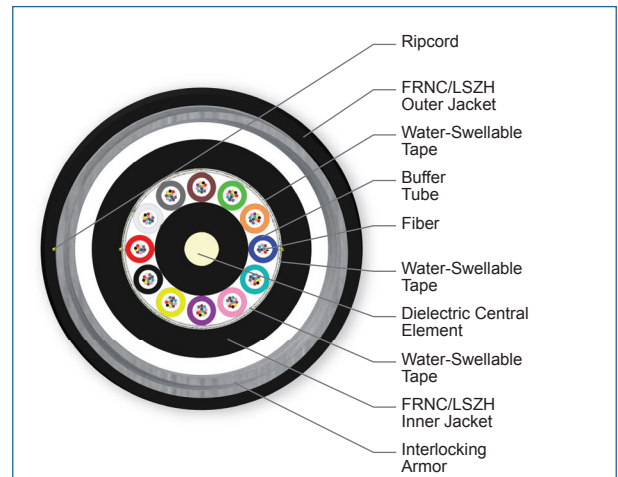
Cross Section of Part Number: 144TUZ-T4190DAN
