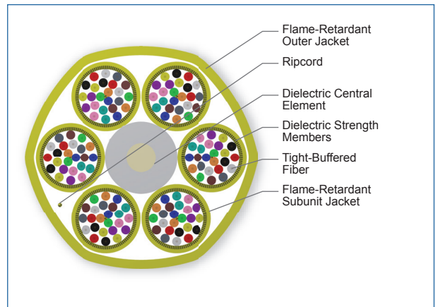
Cross Section of Part Number: 144Z81-Y3131-24
