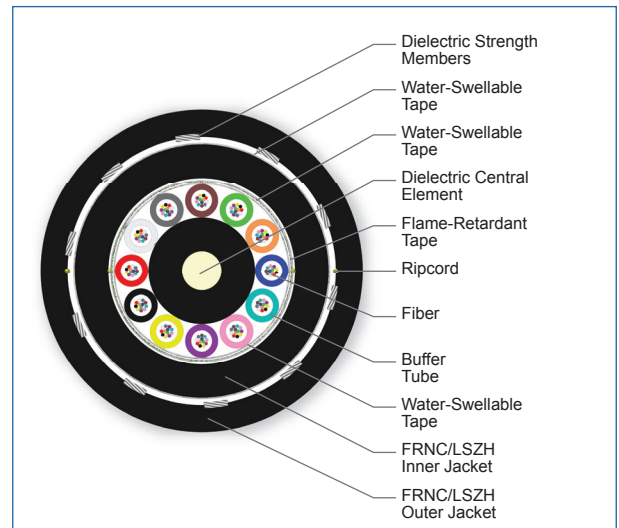
Cross Section of Part Number: 144ZUL-T3601D2M
