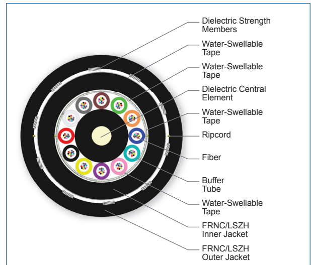
Cross Section of Part Number: 144ZUL-T4601D2N
