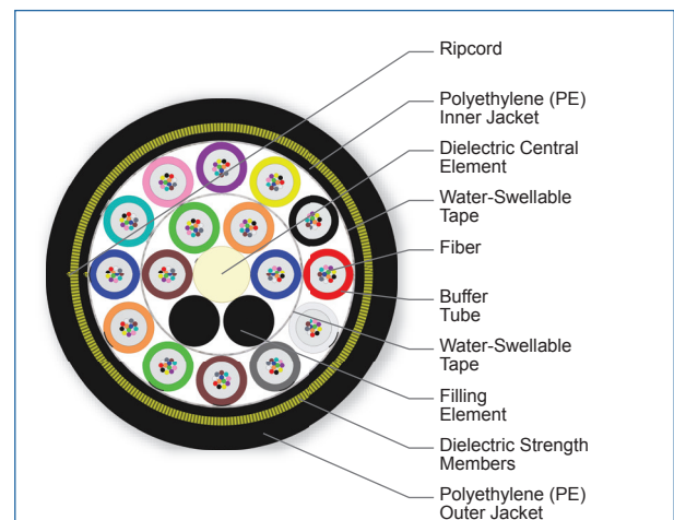
Cross Section of Part Number: 192EAE-T4201A20
