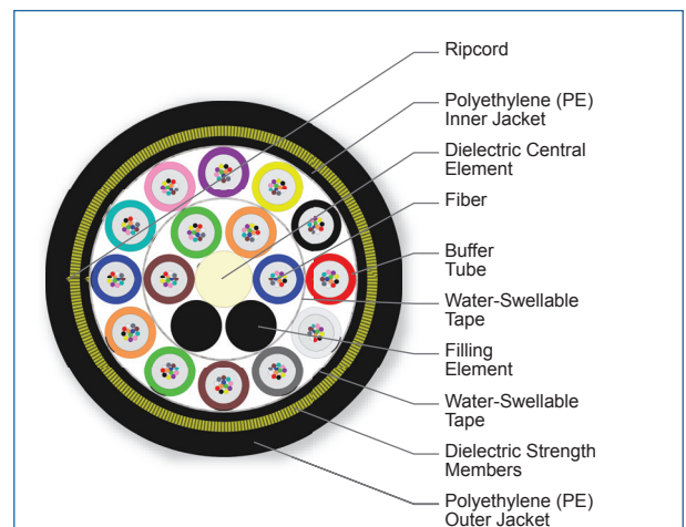
Cross Section of Part Number: 192EAE-T4401A20
