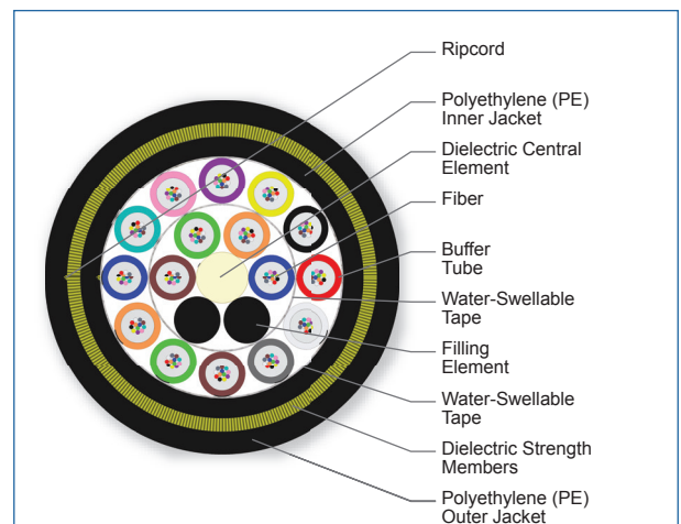
Cross Section of Part Number: 192EAE-T4A01A20
