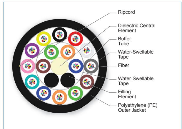
Cross Section of Part Number: 192EU4-T4101D20
