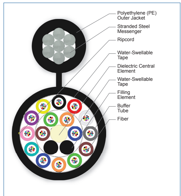
Cross Section of Part Number: 192EUA-T4101D20
