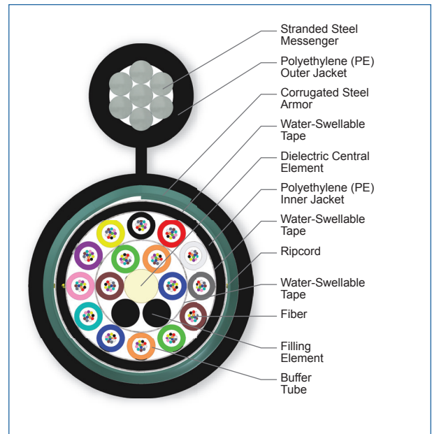
Cross Section of Part Number: 192EUB-T4101D20
