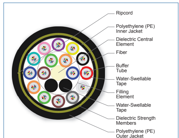
Cross Section of Part Number: 192KAE-T4230A20
