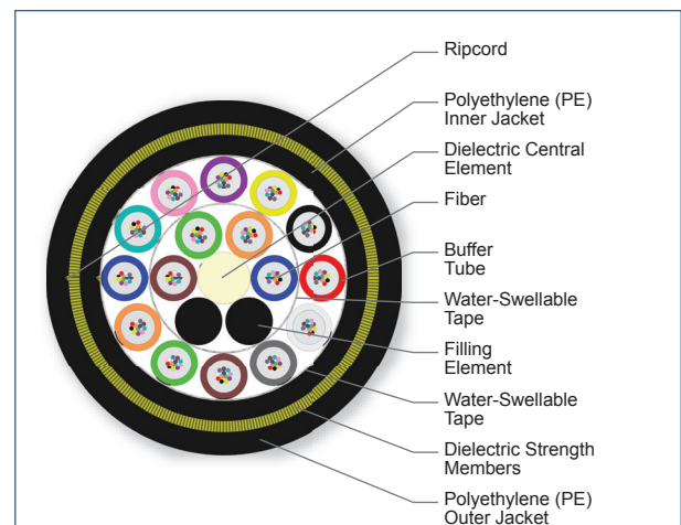
Cross Section of Part Number: 192KAE-T4830A20
