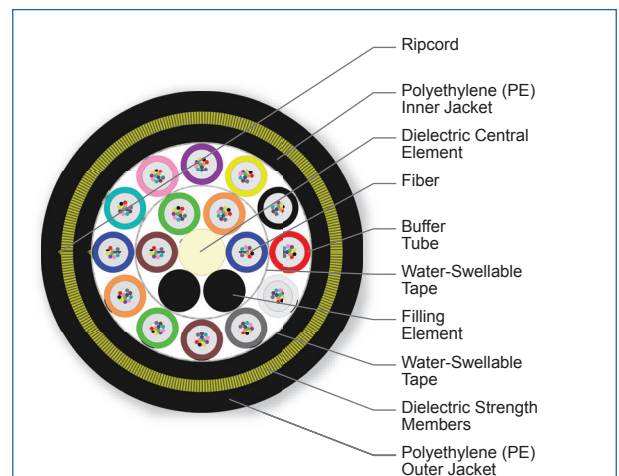
Cross Section of Part Number: 192KAE-T4A30A20
