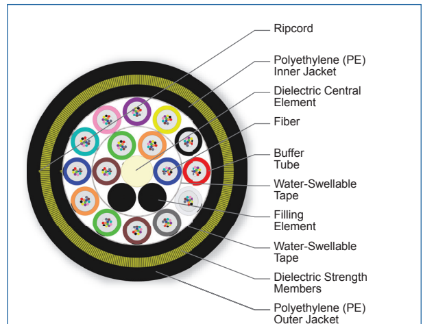
Cross Section of Part Number: 192KAE-T4B30A20
