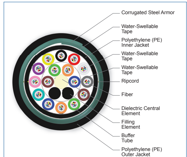
Cross Section of Part Number: 192KU5-T4130A20
