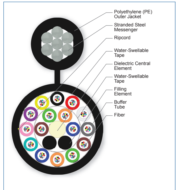
Cross Section of Part Number: 192KUA-T4130D20
