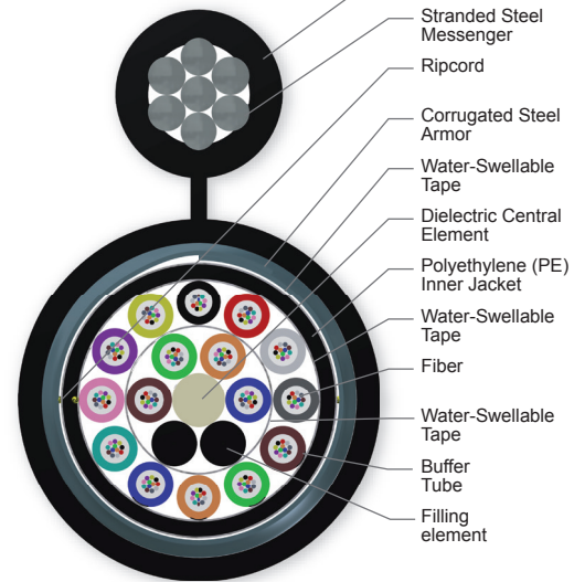
Cross Section of Part Number: 192KUB-T4130A20
