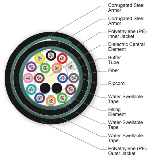
Cross Section of Part Number: 192KUD-T4130A20
