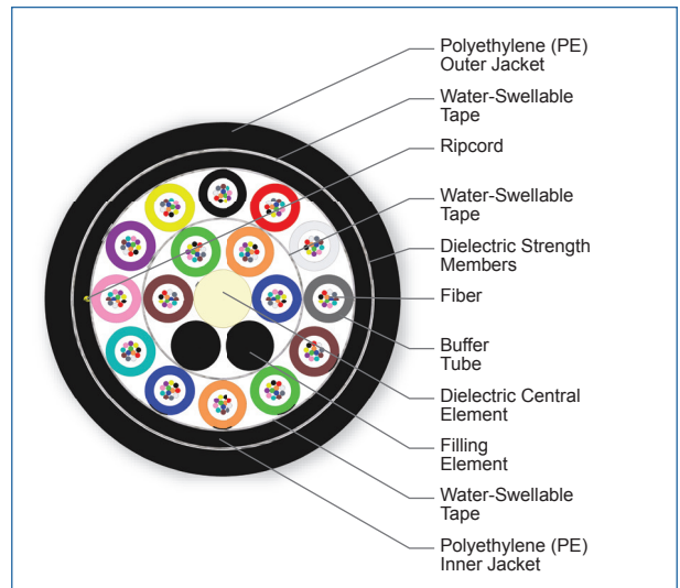
Cross Section of Part Number: 192KUE-T4130D20
