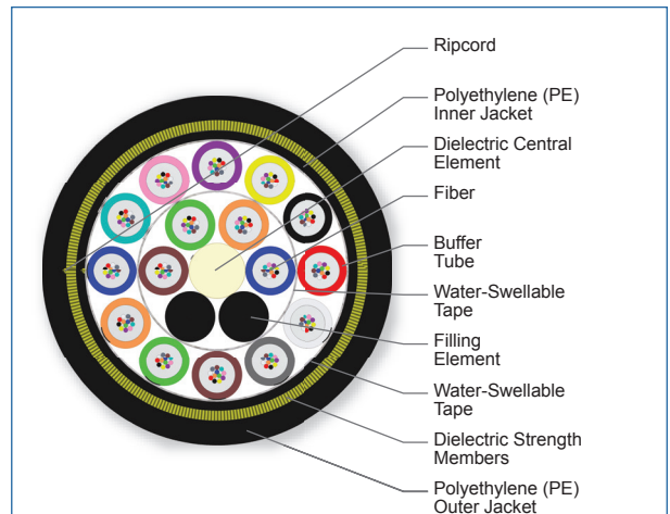
Cross Section of Part Number: 192TAE-T4431A20
