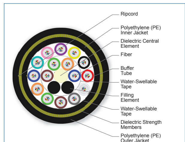
Cross Section of Part Number: 192TAE-T4831A20
