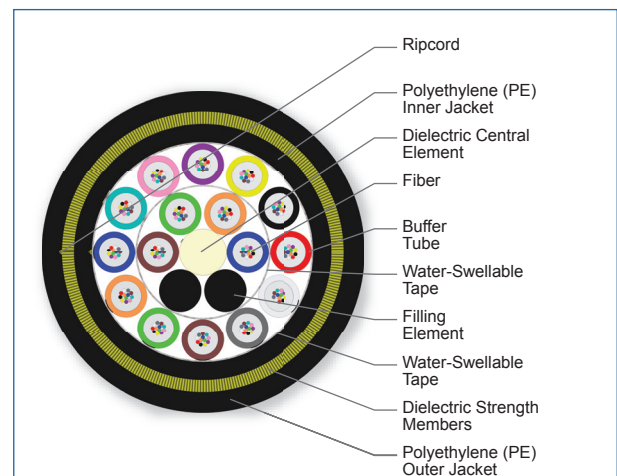
Cross Section of Part Number: 192TAE-T4A31A20
