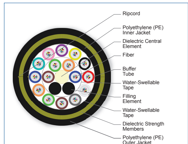
Cross Section of Part Number: 192TAE-T4B31A20
