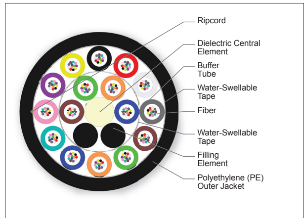
Cross Section of Part Number: 192TU4-T4190D20
