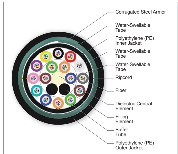
Cross Section of Part Number: 192TU5-T4131A20
