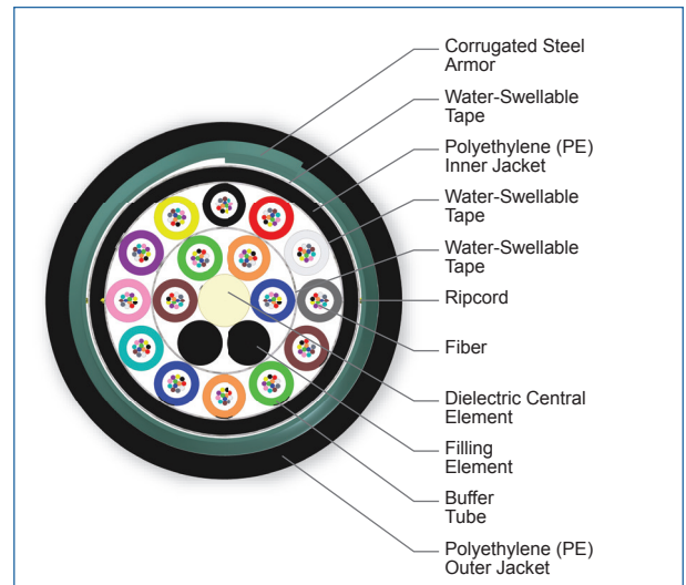
Cross Section of Part Number: 192TU5-T4131D20
